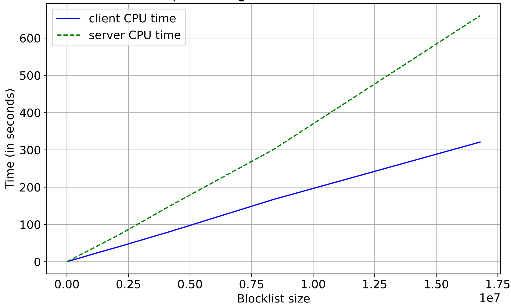
Preprocessing time vs. Blocklist size
